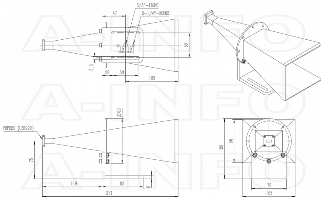
FBP220 Output with L Type Mounting Bracket (Option, P/N: LB-42-25-L2)
