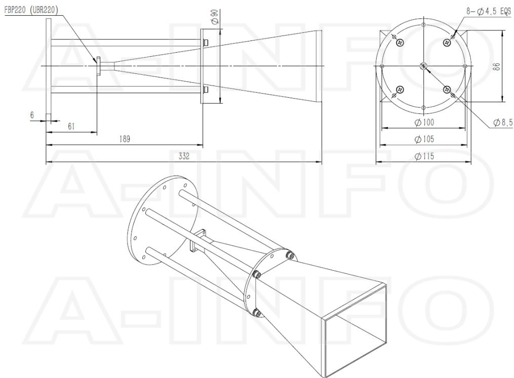
FBP220 Output with Round Mounting Bracket (Option, P/N: LB-42-25-MB2)
